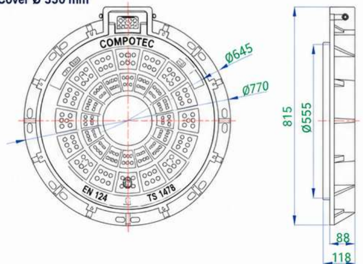
COMPO-MH-200 Series Manhole Cover Ø 550 mm
