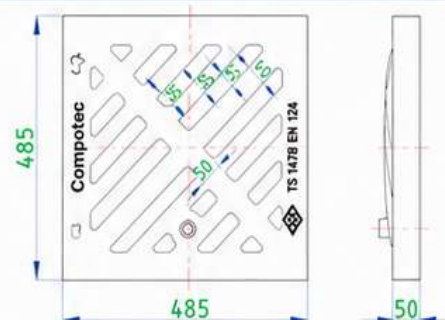
COMPO-G6-202 – Rainwater Grate (485 x 485 mm)
