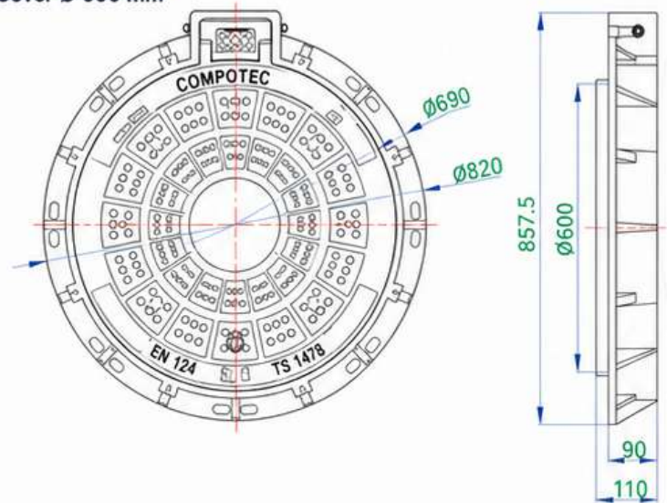
COMPO-MH-100 Series Manhole Cover Ø 600 mm
