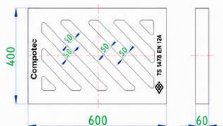
COMPO-G6-203 – Rainwater Grate (400 x 600 mm)
