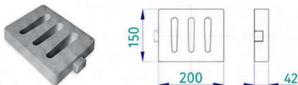
COMPO-TG-201 Tree Grate Adapter (600 x 600 mm)
