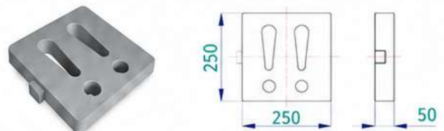
COMPO-TG-202 Tree Grate Adapter (1000 x 1000 mm)
