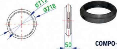
COMPO-LA-100 Pole Base Clamp (10 m)
