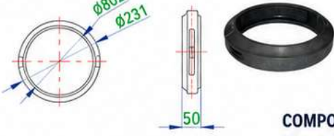
COMPO-LA-200 Pole Base Clamp (12 m)
