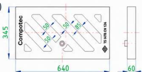
COMPO-G6-201 – Rainwater Grate (640 x 345 mm)
