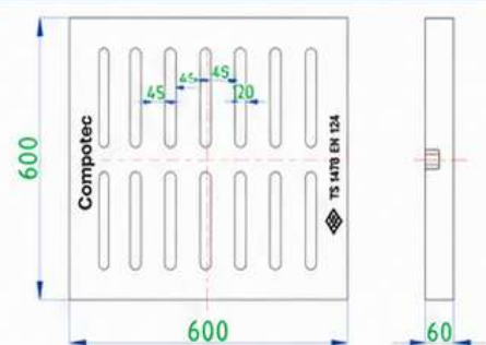
COMPO-G6-204 – Rainwater Grate (600 x 600 mm)
